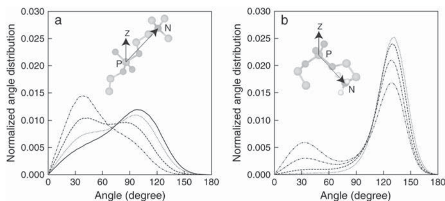
FIGURE 9 Normalized angle distribution for P-N vector for (a) DPPC in Lipid-A to Lipid-D and (b) DPPE in Lipid-B to Lipid-E. Angle is measured with respect to the normal of the bilayer surface (z-axis). Lipid systems are represented by the following lines: solid ( Lipid-A ), dot ( Lipid-B ), dash ( Lipid-C ), dot-dash ( Lipid-D ), and dot-dot-dash ( Lipid-E ). Pictorial representation for P-N vector is shown in the figure.
