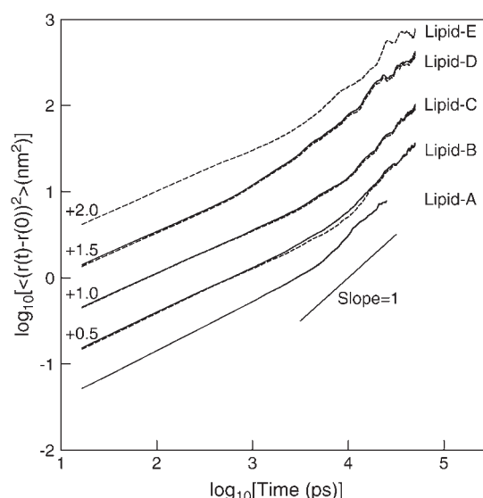
FIGURE 4 Mean-squared displacement of DPPC and DPPE for all lipid systems. Solid and dash-lines represent the displacement of PC and PE lipids, respectively. Short solid line has unity slope. Numbers are the displacement of the lines, shifted for clarity.
